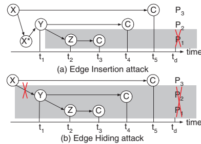
Fig. 3. Attacks
