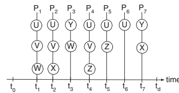
Fig. 4. Paths revealed over time axis
