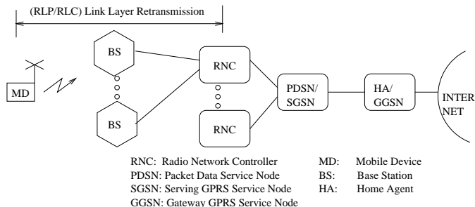
Figure 1: 3G network architecture
