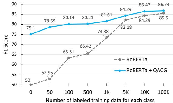
Figure 2: The few-shot learning experiment. The figure shows the F_1 score on FEVER-Symmetric for progressively larger training dataset sizes.
