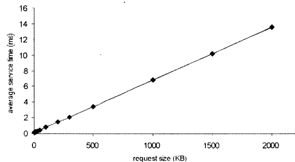
Figure 5. Dispatcher Service Time
