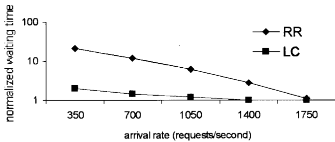
Figure 11. 4-Server Cluster - Normalized Waiting Time
