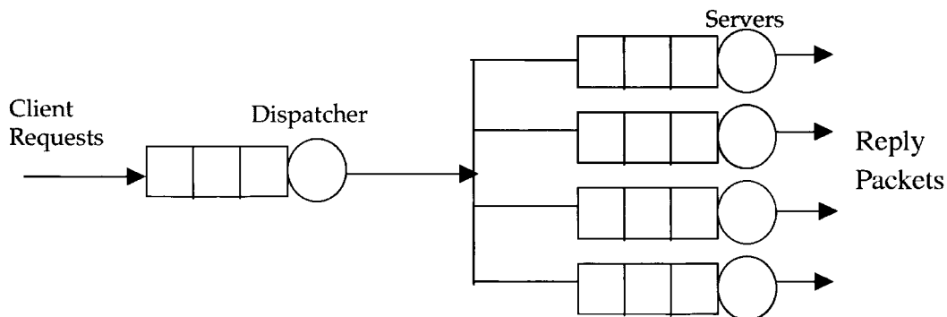
Figure 3. Queuing Model of a Dispatcher-based Cluster of Web Servers
