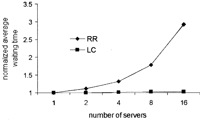
Figure 8. Normalized waiting time (Surge Trace)
