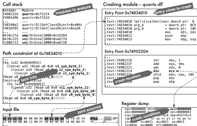
Fig. 2. Crash analysis information for CVE-2010-0718
