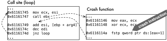
Fig. 5. Example of loop-dependent crash in Real Player
