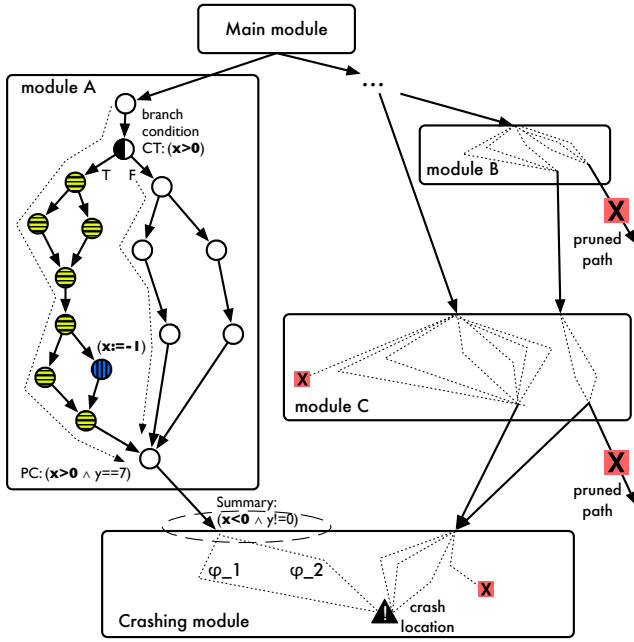
Fig. 3. Schematic module dependence graph with paths to crashing module
