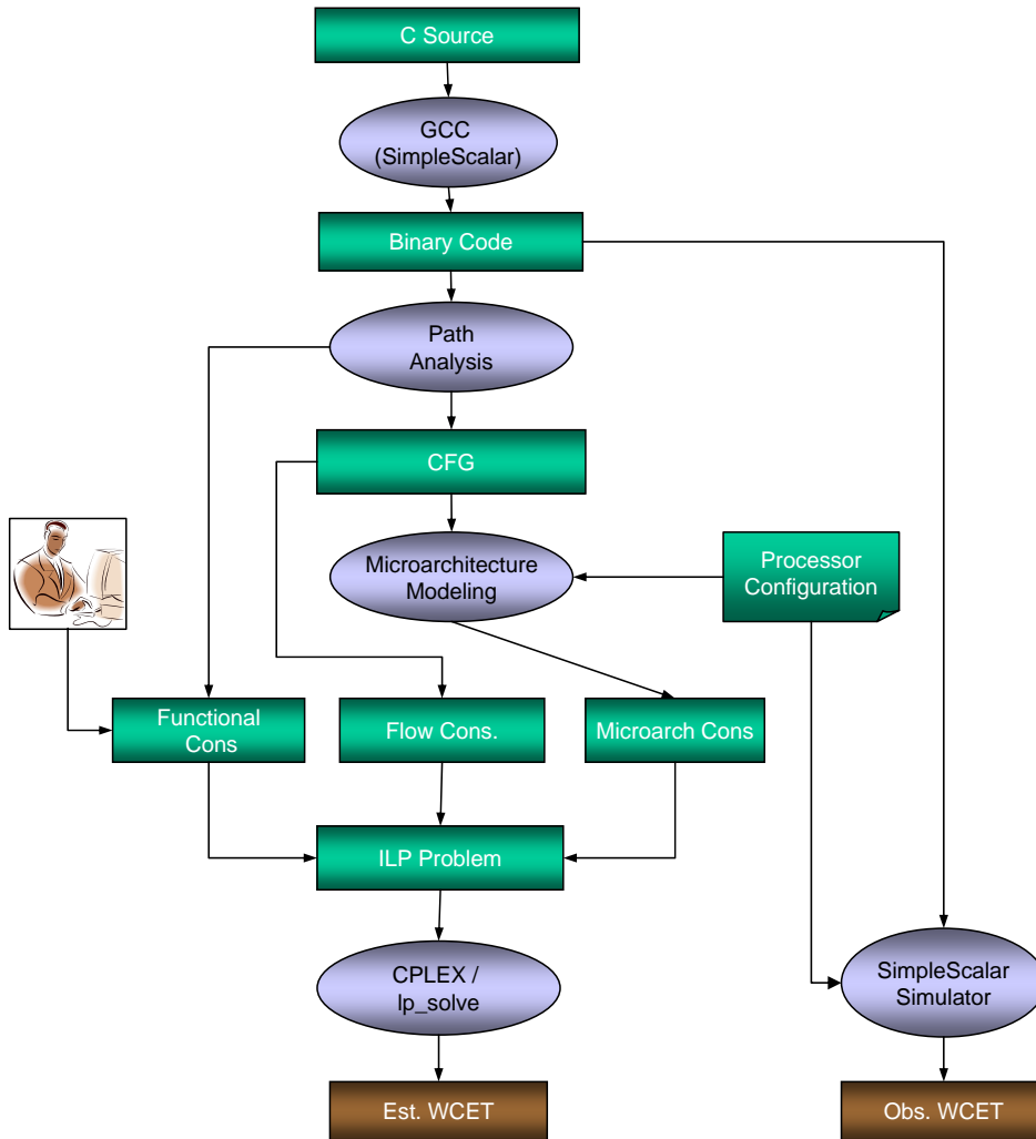
Fig. 1. Workflow of the Chronos timing analyzer
