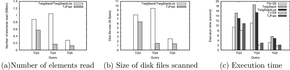
Figure 8: TwigStack, TwigStackList, TJFast on TreeBank
