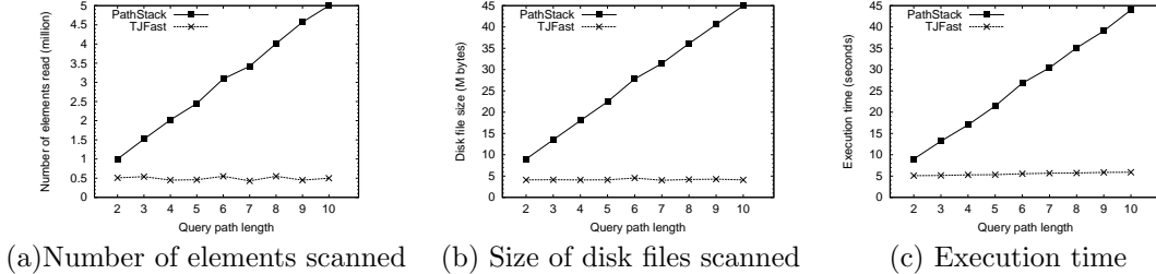
Figure 6: PathStack versus TJFast using random data
