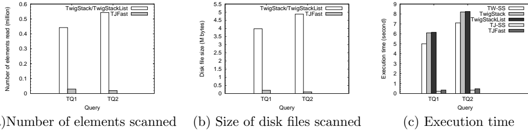
Figure 7: TwigStack, TwigStackList versus TJFast on DBLP
