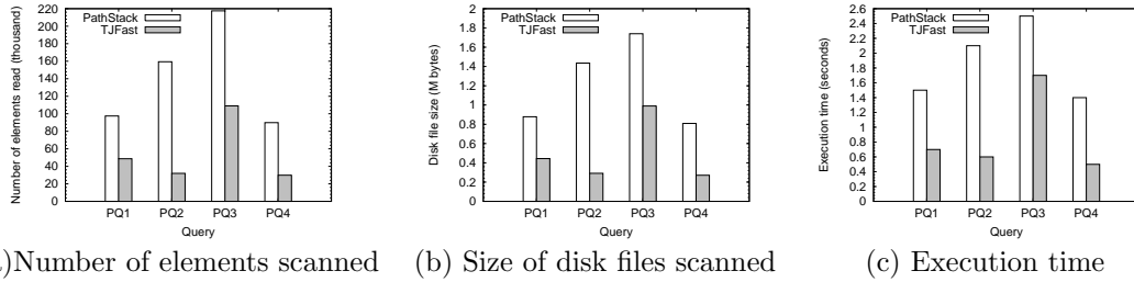
Figure 5: PathStack versus TJFast using XMark data
