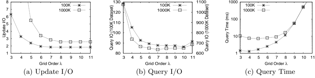
Figure 8: Grid Granularity
