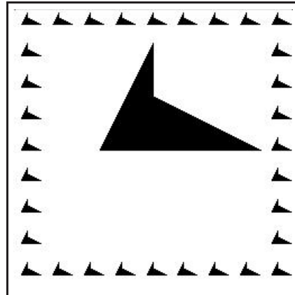
(b) show(persian(nova_bb, 9));
