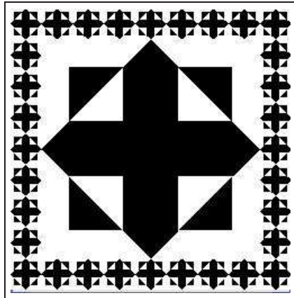
(a) show(persian(make_cross(rcross_bb), 9));
