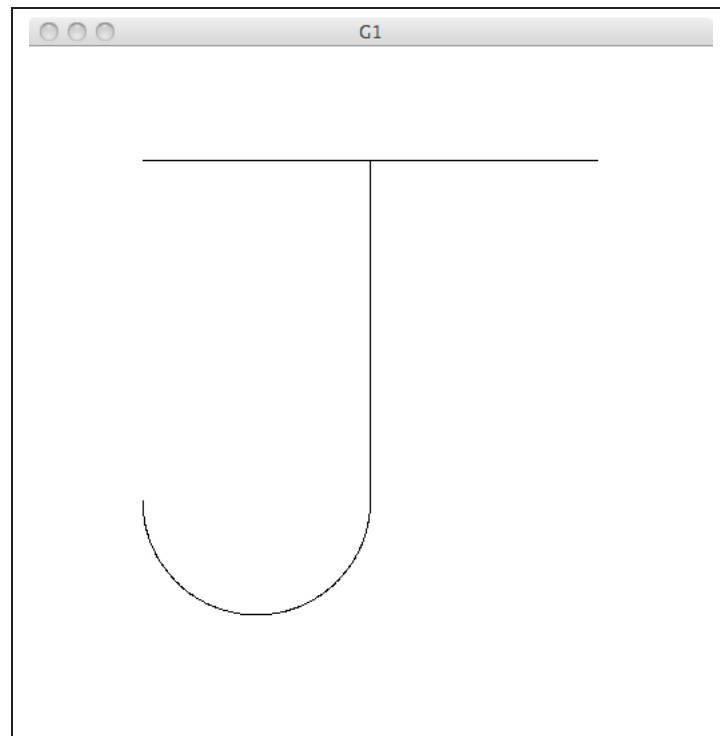
Figure 1: draw_connected(1000)(J);
