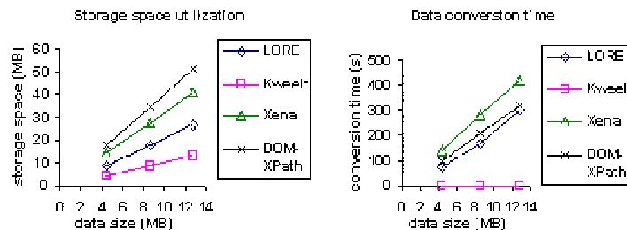
Fig. 1. Space Utilization and Data Conversion Time
