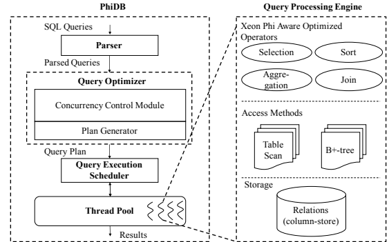
Figure 1: System overview of PhiDB
