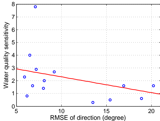
Fig. 16: The RMSE of direction prediction corresponding to the water quality sensitivity for each mobile test location. The red line is the linear fitting curve of the scatter points.
