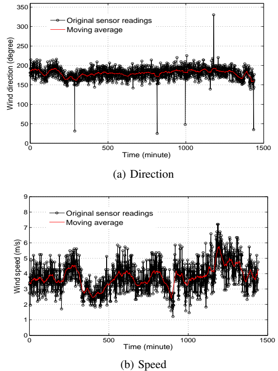
Fig. 13: Time series of wind direction and speed from 00:00 to 23:29 on 1 September 2013
