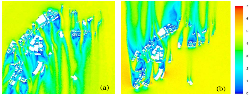
Fig. 6: CFD modeling results of wind velocity (m/s) distribution at 1.5 meter height with an incoming atmospheric flow from North (a) and South (b)
