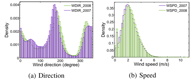
Fig. 4: Wind Density for two consecutive years (2007 and 2008) collected at Marina Bay meteorological station.
