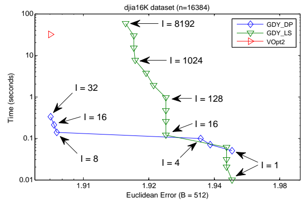
Figure 5: GDY_LS vs. GDY_DP, B = 512 : DJIA
