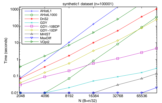
Figure 3: Runtime vs. n , B = \frac{n}{32} : Synthetic
