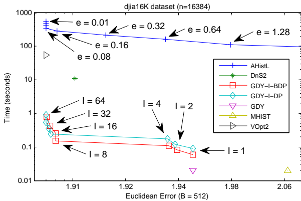
Figure 4: Tradeoff Delineation, B = 512 : DJIA
