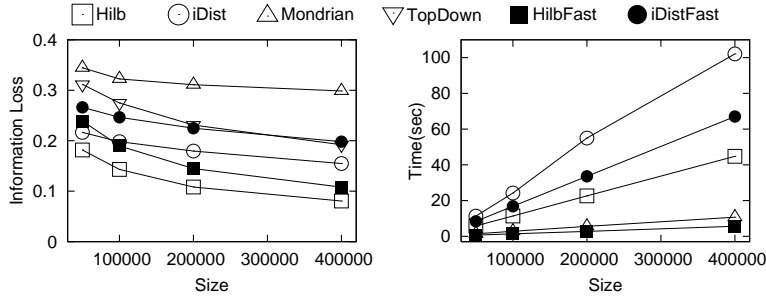
Fig. 23. Privacy-Constrained k -anonymization, variable N
