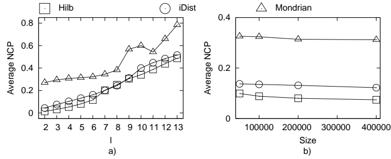
Fig. 30. Privacy-Constrained l -diversification, Average NCP metric
