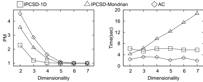
Fig. 33. Accuracy-Constrained \ell -diversity, variable Q_T dimensionality
