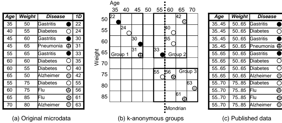
Fig. 1. k -anonymization example ( k=4 )
