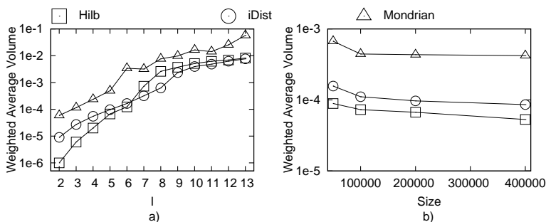
Fig. 31. Privacy-Constrained \ell -diversification, Weighted Average Volume metric
