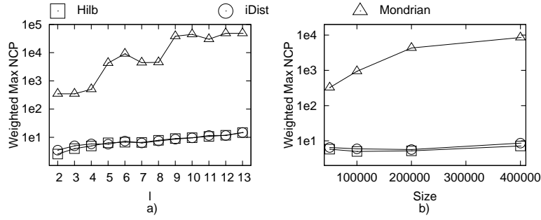
Fig. 29. Privacy-Constrained l -diversification, Weighted Maximum NCP metric
