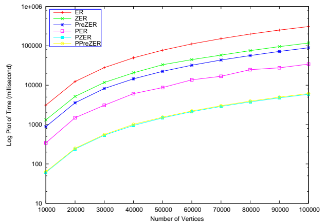
Figure 15: Runtime for varying graph size, p = 0.1
