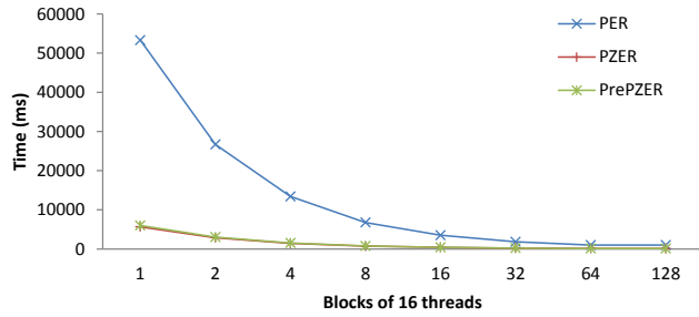
Figure 12: Runtime of the parallel algorithms for varying thread-blocks for \Gamma_{v=10K, p=0.1} graphs
