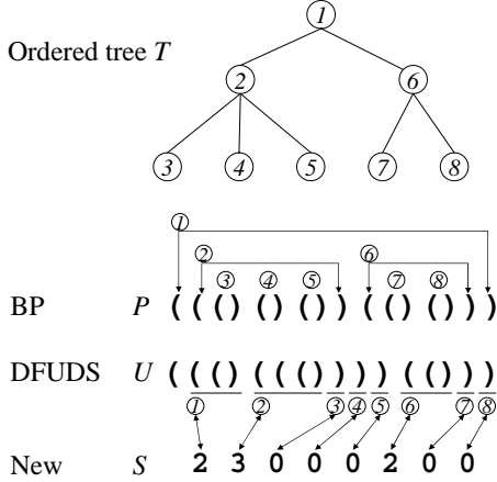
Figure 1: Succinct representations of trees.
