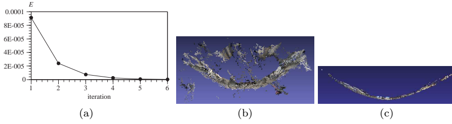
Fig. 1 Robust surface fitting. (a) Convergence curve. (b) 3D points around a curved surface. (c) Inliers identified by the robust fitting algorithm lie very close to the fitted surface.
