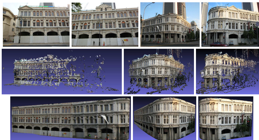
Fig. 6 Reconstructed mesh models of building 2. (Row 1) Sample images from various views. (Row 2) Point clouds recovered by PMVS and (Row 3) reconstructed textured mesh model at various viewing angles.
