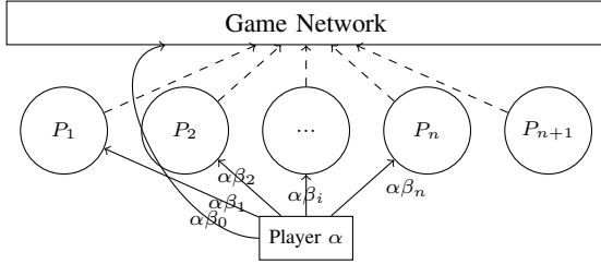
Fig. 1: The CPS game setup of n + 1 pools with respect to a player with \alpha fraction of total computational power in the game.
