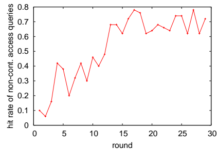
Figure 4: Non-continuous access query hit rate over time
