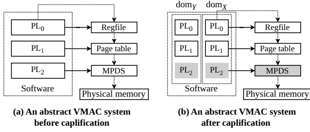
Figure 2: A VMAC-based system before and after caplification. Solid arrows indicate which software components control which architectural structures. Dotted arrows indicate the pathway of a memory access from PL 0 . Shaded areas represent capability-aware software components or structures.
