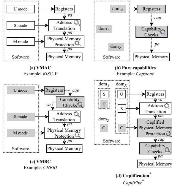
Figure 1: Comparison of hardware isolation mechanisms, using RISC-V as an example. Solid arrows represent writable permissions. Dotted arrows represent the pathways for software to access physical memory. Shaded regions represent structures that contain capabilities or capability-aware software components. The asterisked mechanism (d) is our work. Labels va , pa , and cap represent virtual addresses, physical addresses, and capabilities, respectively. The magnifying glass icon (Q) indicates locations of checks on the memory access.
