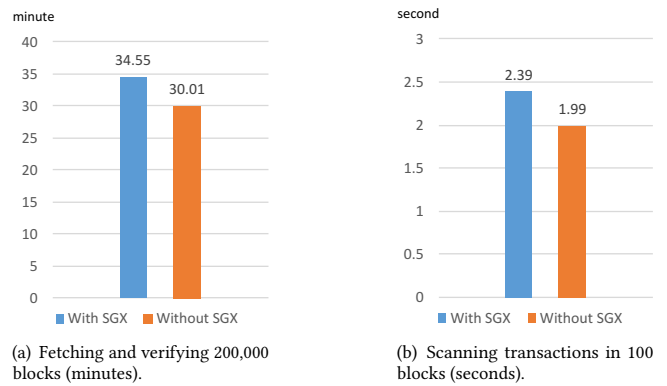
Figure 3: Measured time for fetching blocks and scanning transactions with/without SGX.
