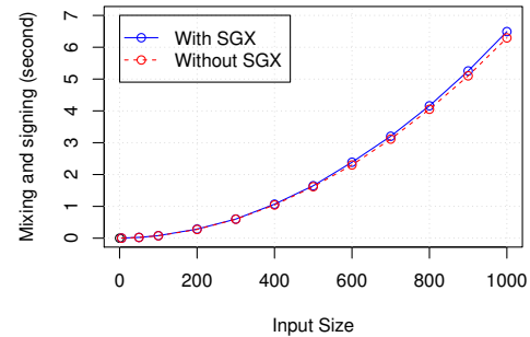
Figure 4: OBSCURO signing and mixing time with/without SGX.
