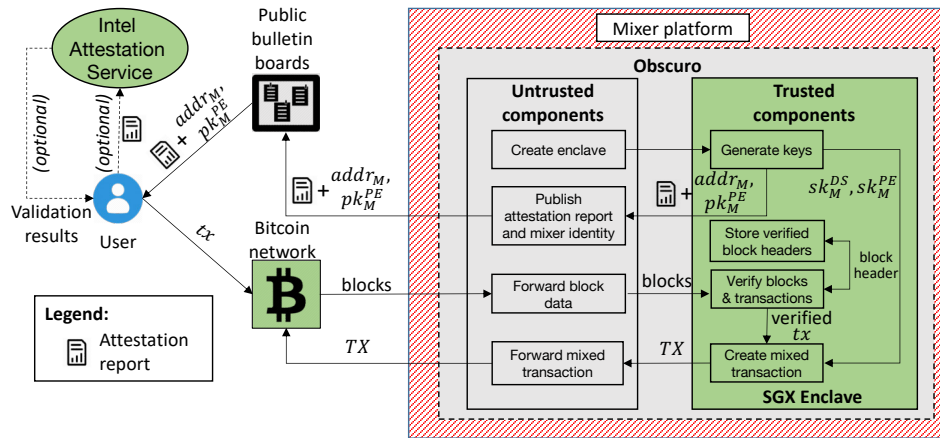
Figure 1: The OBSCURO architecture. Components in the green background are trusted, while the ones in the gray background are untrusted. The adversary controls the components in the red stripe background.
