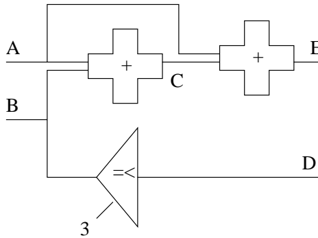
Figure 7: Circuit Analysis.
