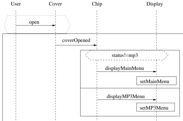
Figure 1. Phone System Scenario: OpenCover
