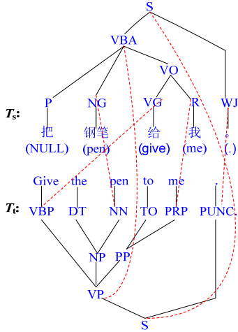
Figure 1: Sub-tree alignment as referred to Node alignment
