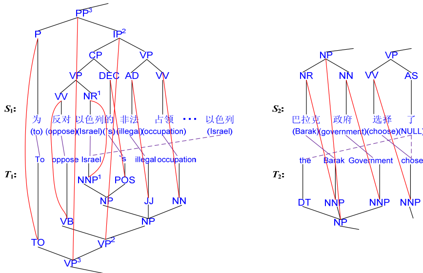
Figure 3: Comparison between Sub-tree alignment results and Word alignment results
