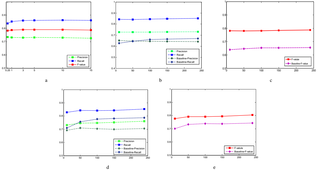
Figure 2: a. Precision/Recall/F-score for various amount of training data ( k ). b~e. Various amount of data to train word alignment b. Precision/Recall for HIT test set. c. F-score for HIT test set. d. Precision/Recall for FBIS test set. e. F-score for FBIS test set.
