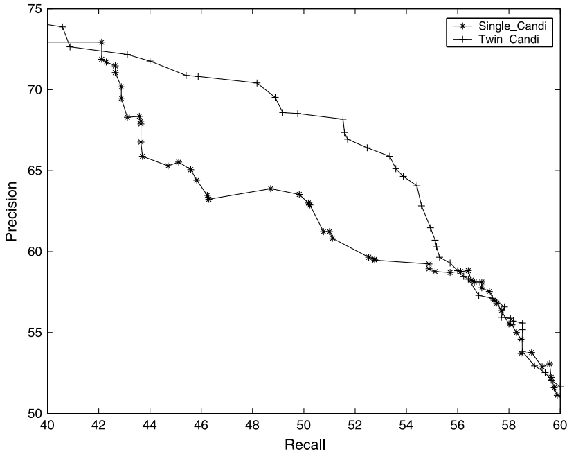
Figure 4 Various recall and precision rates for the coreference resolutions systems (non-pronoun).
