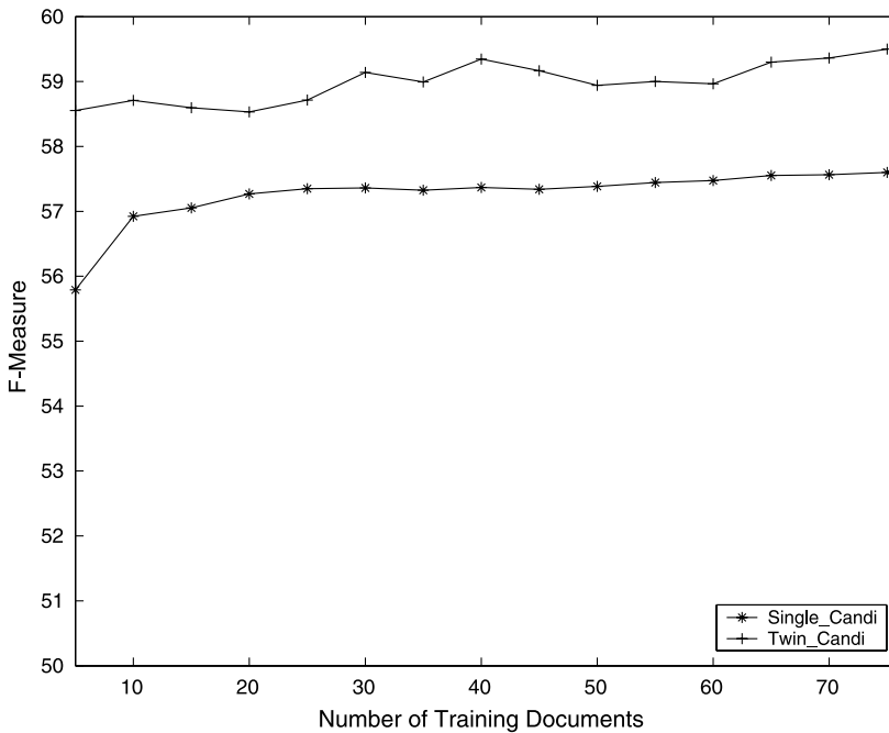
Figure 7 Learning curves for coreference resolution systems (non-pronoun).
