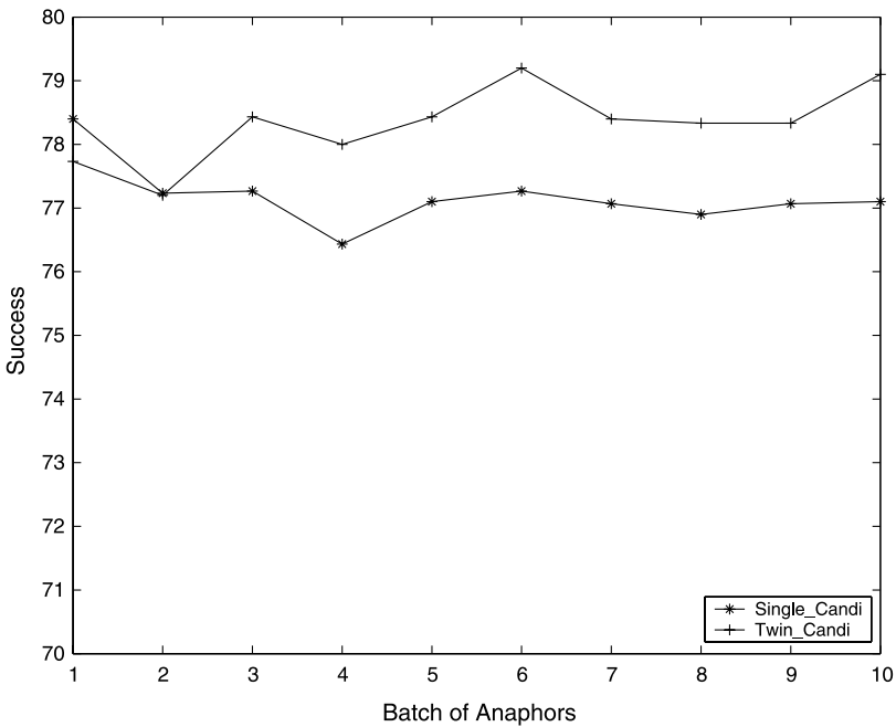
Figure 3 Learning curves of the systems with different models for pronominal anaphora resolution in the NPaper Domain (120 anaphors per batch).
