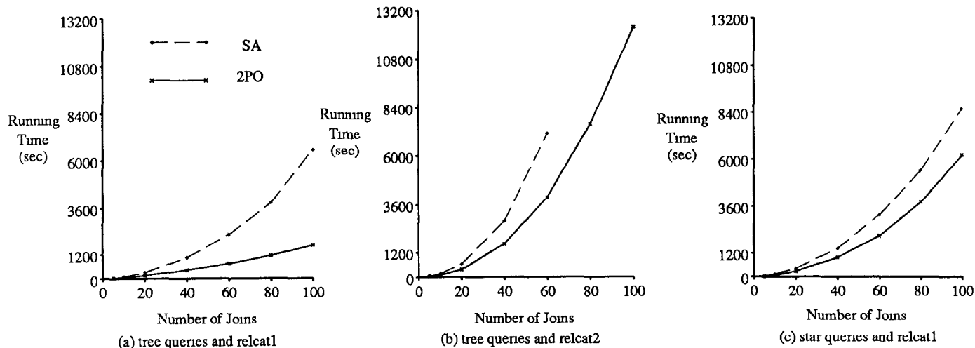
Figure 3.5• Average running time of SA and 2PO
