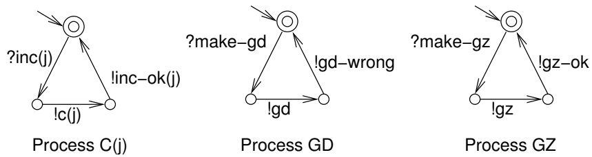
Fig. 12. Description of processes GD , GZ , C(j) in phase (iii)
