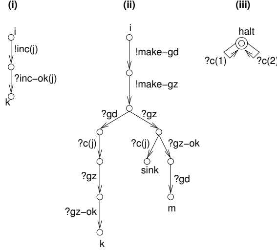
Fig. 10. Transitions of process A in phase (ii)
