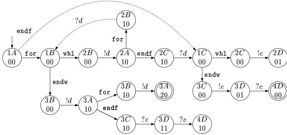
Fig. 15. The tree W in Thm. 11 for the system in Fig. 14.
