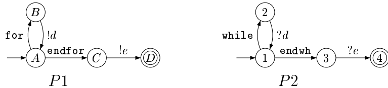
Fig. 14. A data-branching system.
