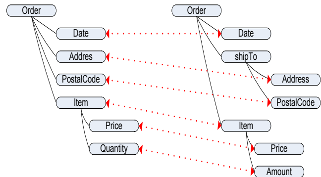
Figure 1 Source and target schema trees with final matching. Red dotted lines connecting two nodes represent they are matched.
