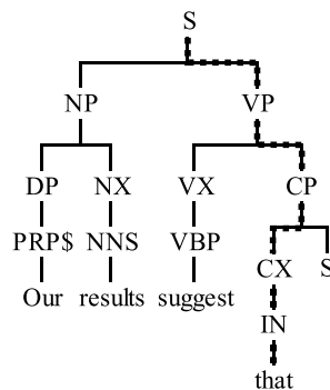
Fig. 2. Partial lexical parse tree of a sentence starting with a causal trigger.
