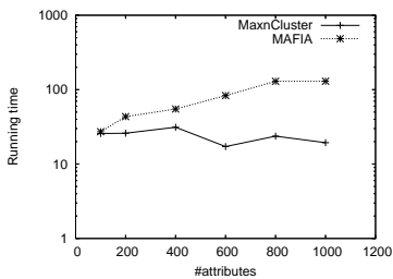
(b) Varying #attributes A
