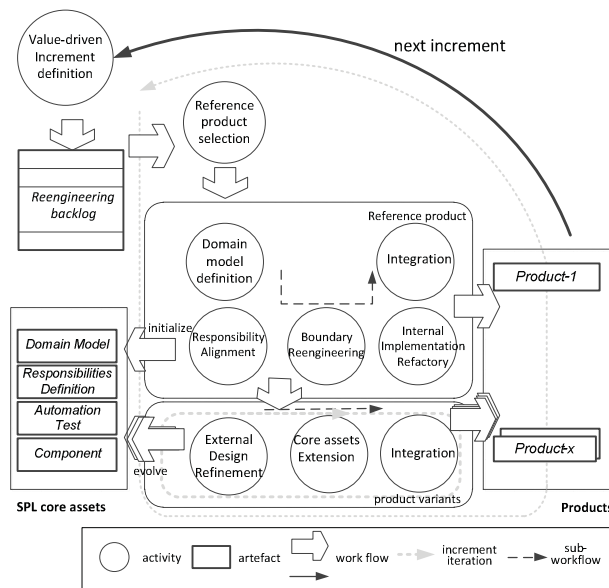
Figure 2. Process overview of the IXM-PF reengineering project
