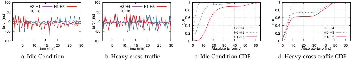
Figure 16: Error in DPTP Switch-to-Host synchronization
