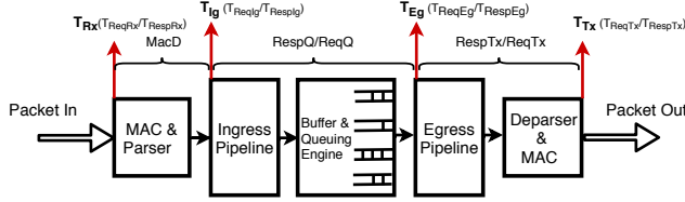
Figure 2: Portable Switch Architecture [28]
