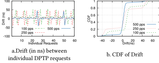
Figure 13: Drift captured at S6 for different DPTP synchronization intervals
