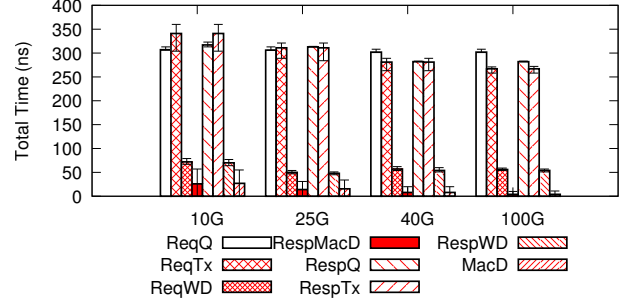
Figure 4: Delays for various link-speeds (idle links)
