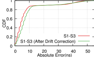
Figure 14: DPTP w/ and w/o linear drift correction
