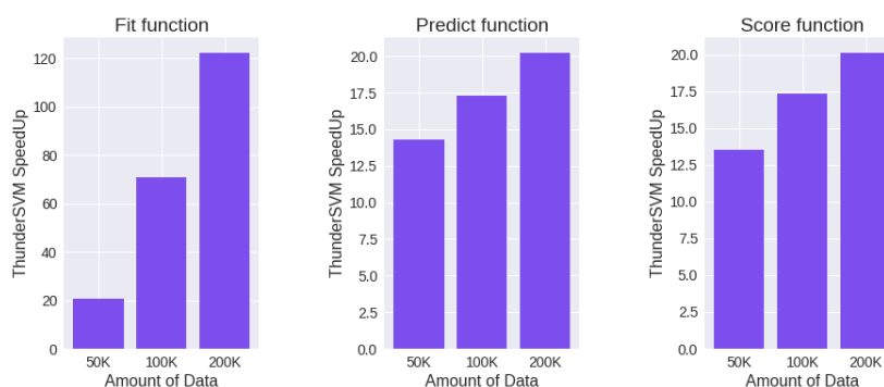
Performance Speedup for ThunderSVM
