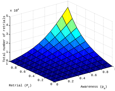
Figure 7: Total number of retrials as a function of retrial probability p_r and awareness p_a
