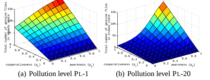
Figure 6: Number of genuine files in steady state as a function of cooperativeness and awareness
