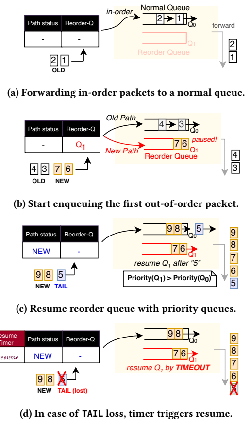
Figure 9: ConWeave packet reordering. A single flow needs only one FIFO queue to reorder packets. ConWeave DOES NOT rely on the packet sequence numbers to reorder them. Instead, we differentiate the order of the packets through the REROUTED and TAIL flags.
