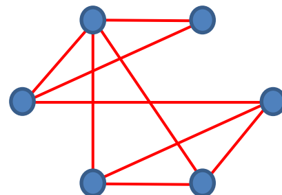
Fig. 10c. The complementary graph
