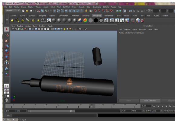
Marker Model
