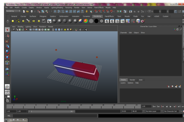
Eraser Model
