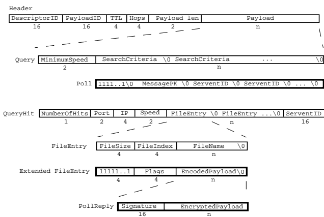
Figure 4: A description of P2PRep messages
