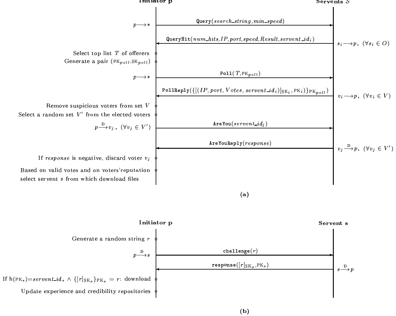
Figure 3: Sequence of messages and operations in the enhanced polling protocol (a) and interactions with the selected servent (b)
