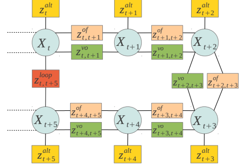
Fig. 9. g2o hypergraph representation of our pose-graph SLAM problem.
