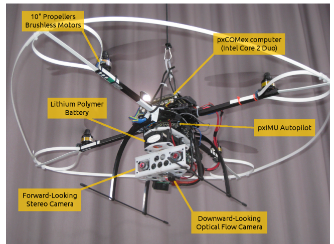
Fig. 1. Our PIXHAWK quadrotor system.
