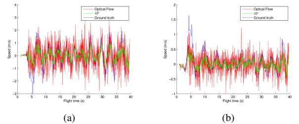
Fig. 3. Results of x and y velocities from the Kalman filter.
