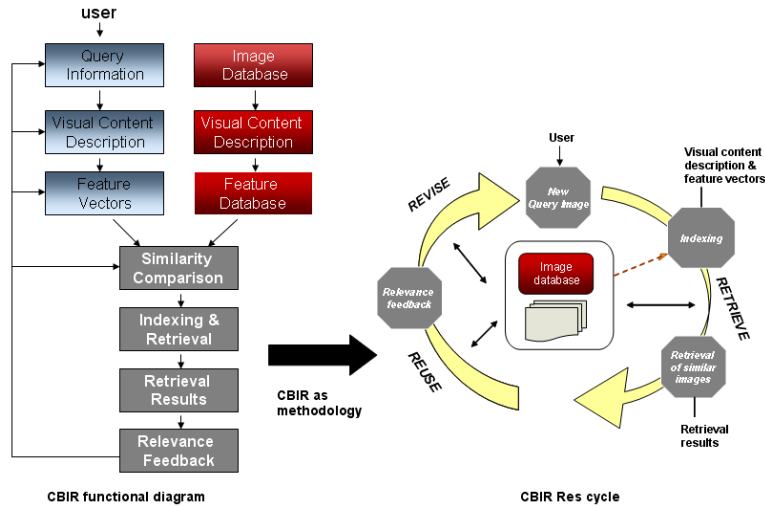
Fig. 4. CBIR methodology
