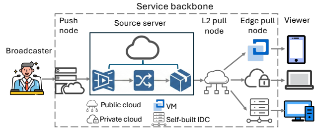
Figure 1: An end-to-end view of LiveNet architecture.
