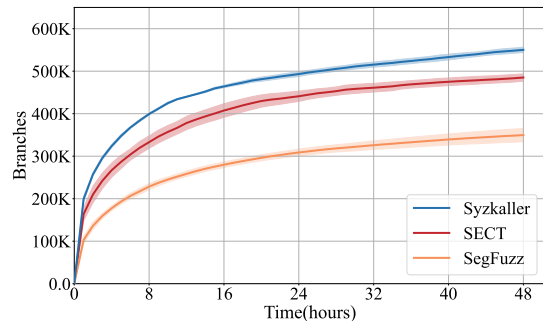
Figure 3: Code coverage achieved by Syzkaller, SegFuzz and SEXT (N=10).
