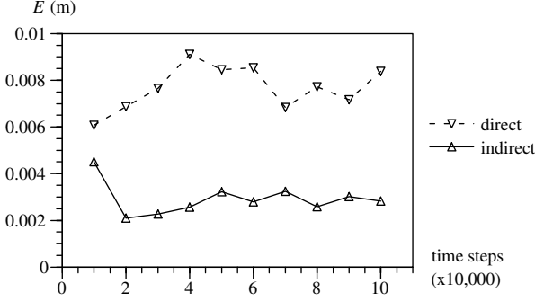
Figure 4: Mean positioning error at various training stages.
