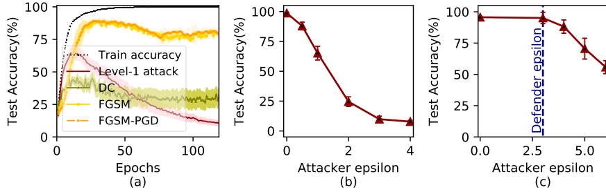
Figure 4: (a) Learning curves for various attacks on MNIST against level-0 defender, and test accuracy for our level-1 attack on MNIST with varying \epsilon_{\text{atk}} against (b) level-0 and (c) level-1 defenders. Lower accuracy reflects better attack. Error bars indicate standard deviations over 5 runs.
