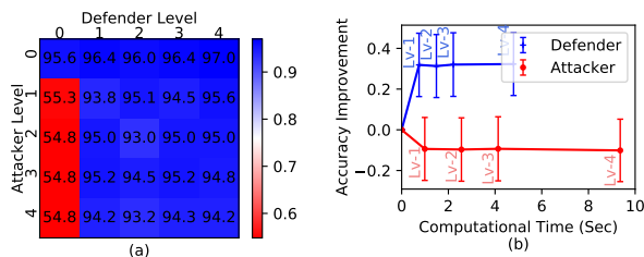
Figure A.10: (a) Mean test accuracy on 2-class ImageNet (i.e., same as Fig. 7c in Sec. 6.3). (b) Graph of mean accuracy improvement (over null strategy) vs. time needed to compute strategies given a minibatch of 2-class ImageNet.
