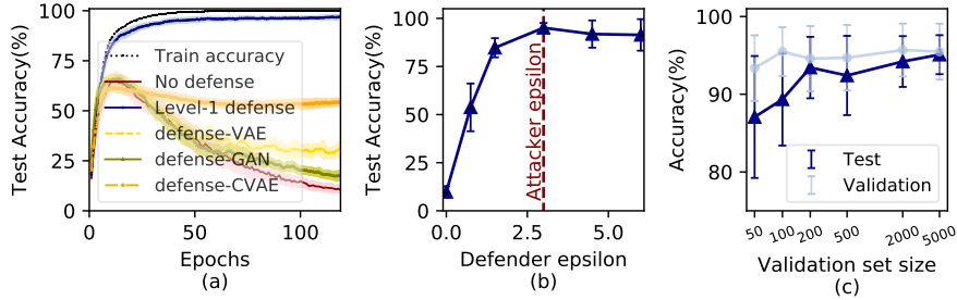
Figure 5: (a) Learning curves for various defenses on MNIST against level-1 attacker, and test accuracy for our level-1 defense on MNIST with varying (b) \epsilon_{\text{def}} and (c) size of validation set known to the defender. Higher accuracy reflects better defense performance. Error bars indicate standard deviations over 5 runs.
