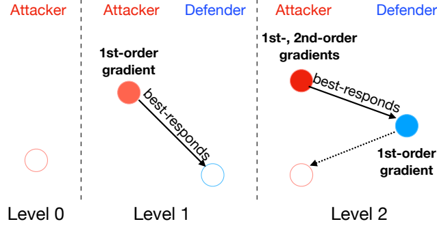
Figure 2: Illustration of how a level- k = 0, 1, 2 attack strategy is computed under the LK model for R2T2 framework.
