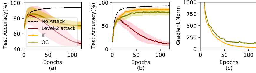
Figure 6: Test accuracy of (a) binary classifier and (b) CNN classifier for 3 different level-2 attack methods, and (c) gradient norm \sum_{x \in \mathcal{D}_t} \|\nabla_{\theta} \mathcal{L}_{\theta_t}(x)\|_2 for CNN classifier. The error bars indicate standard deviations over 10 runs.
