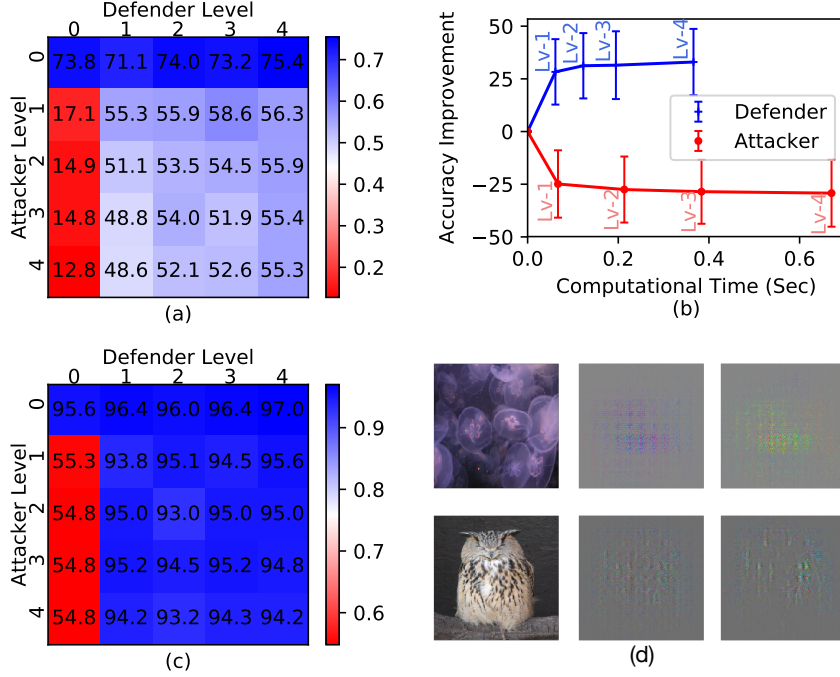
Figure 7: (a) Mean test accuracy (%) on CIFAR-10. (b) Graph of mean accuracy improvement (over null strategy) vs. time needed to compute the strategies given a minibatch of CIFAR-10. (c) Mean test accuracy for 2-class ImageNet. (d) From left to right are visualizations of the original sampled images from ImageNet, perturbations from level-1 attacks, and transformations from level-1 defenses, respectively (color rescaled for viewing).
