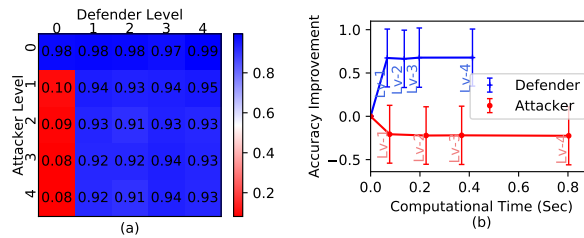
Figure A.9: (a) Mean test accuracy (%) on MNIST. (b) Graph of mean accuracy improvement (over null strategy) vs. time needed to compute the strategies given a minibatch of MNIST.
