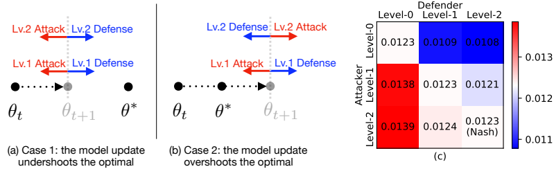
Figure 3: Behaviors of level-1 and level-2 players when the original updated model parameters \theta_{t+1} (i.e., not subject to attack/defense) (a) undershoots and (b) overshoots the optimal parameters \theta^* . (c) shows mean test loss after 30 training iterations.
