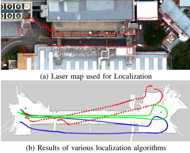
Fig. 7. Comparison of various localization schemes
