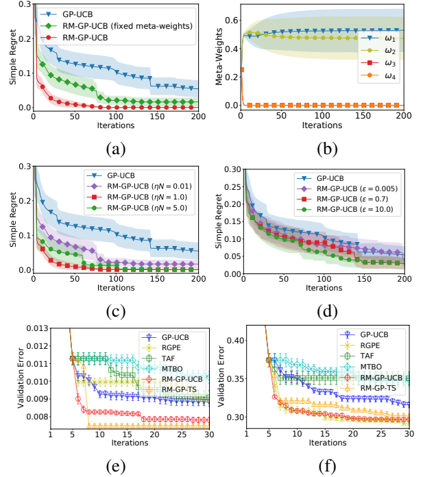
Figure 1: (a) The simple regret and (b) meta-weights optimized by RM-GP-UCB. The impact of (c) \eta and (d) \epsilon . Best validation error of CNN for (e) MNIST and (f) CIFAR-10.
