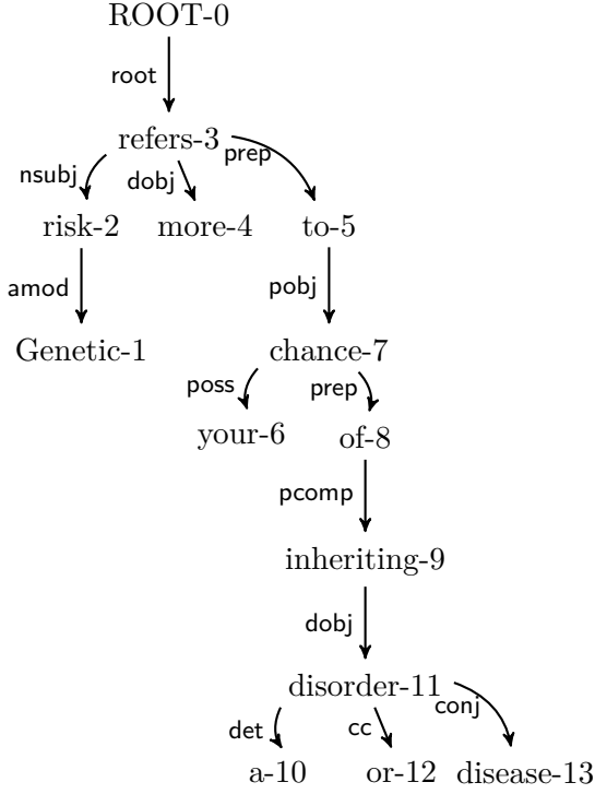
Figure 1: Basic dependencies.
