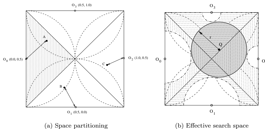
Fig. 7. Using (centers of hyperplanes, closest distance) as reference point.
