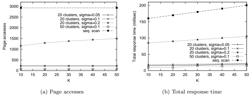
Fig. 25. Effects of different data distribution, clustered data
