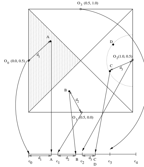
Fig. 3. Mapping of data points
