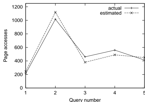
Fig. 31. Evaluation of the histogram-based cost model
