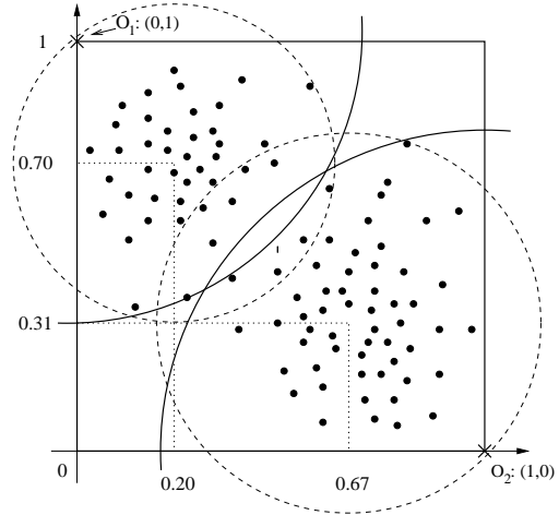
Fig. 11. Cluster edge points as reference points
