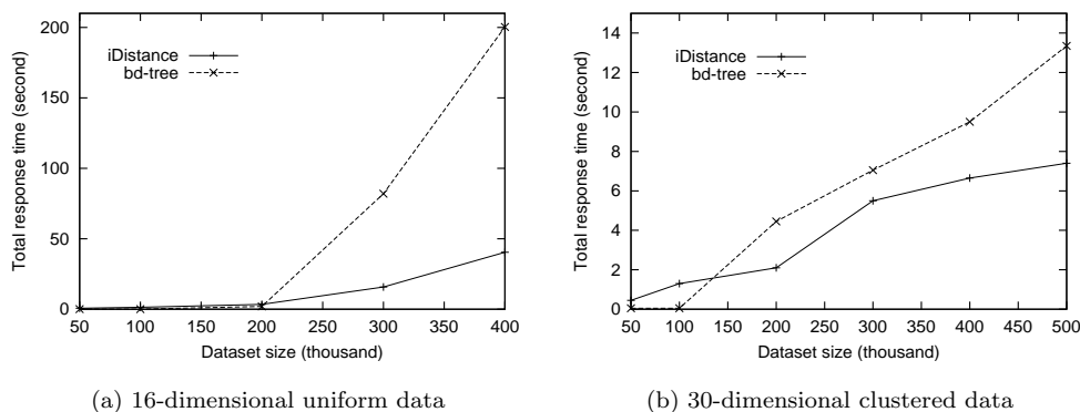
Fig. 29. Comparison with a main memory index: bd-tree
