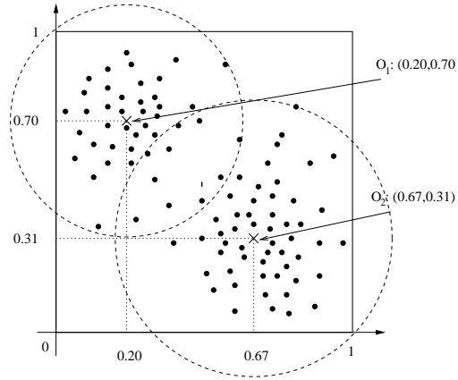
Fig. 10. Cluster centers and reference points
