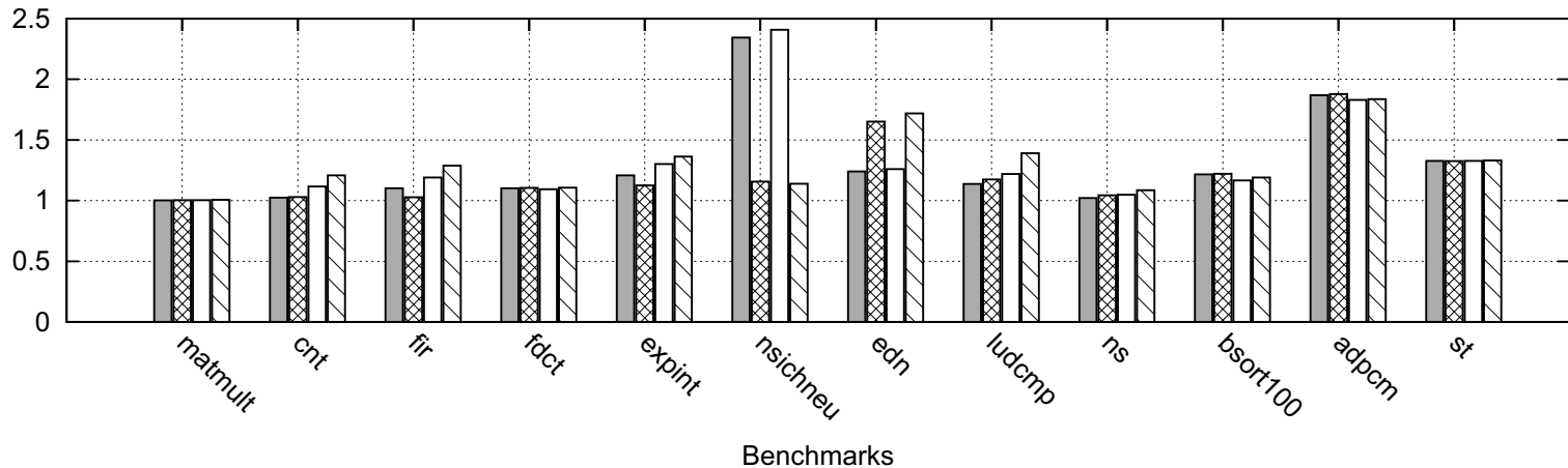
WCET overestimation in presence of shared bus
